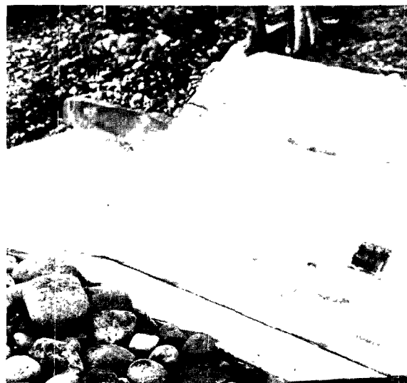
FIGURE 28.—Completed prefabricated trapezoidal supercritical-flow flume.
