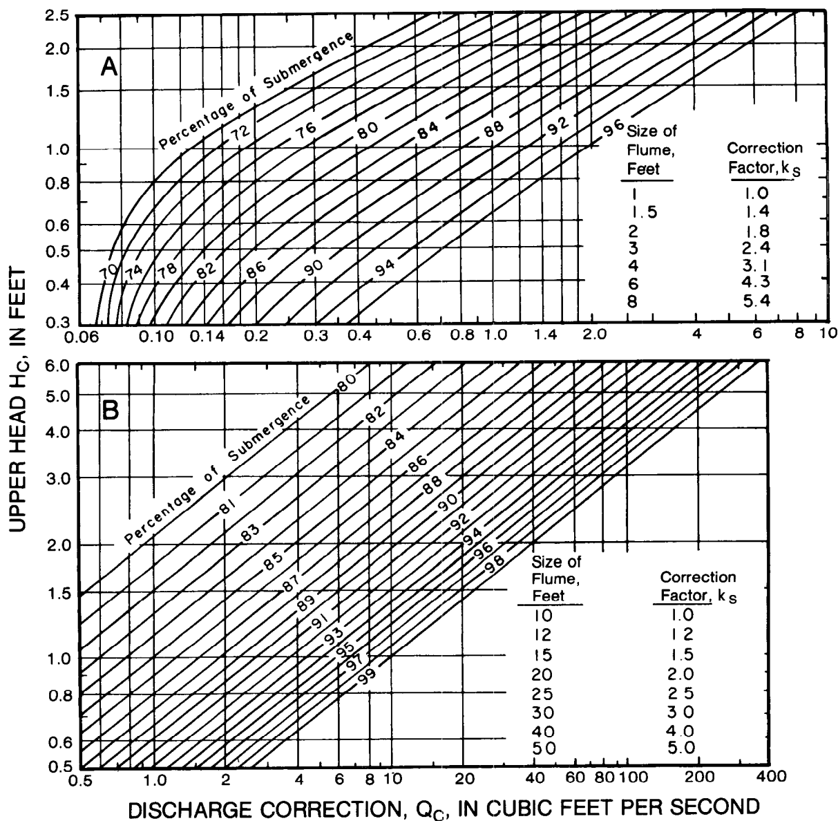
FIGURE 10.—Correction factors for submerged flow through A, 1- to 8-foot, and B, 10- to 50-foot Parshall flumes.
