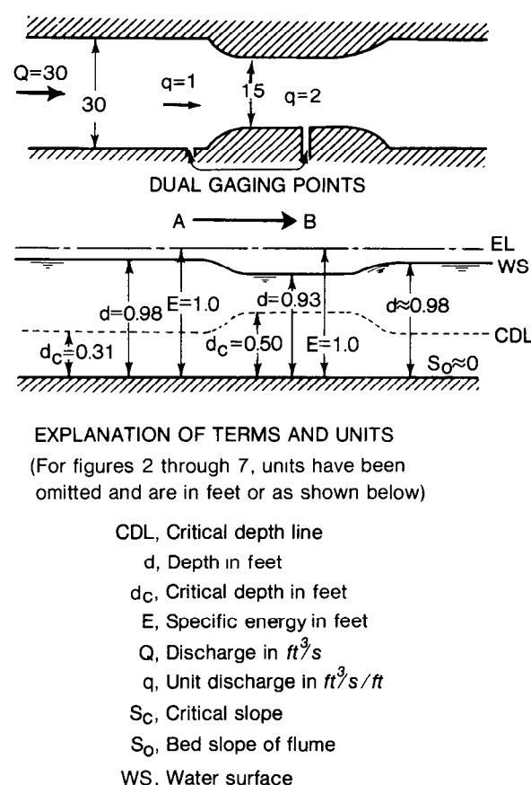
FIGURE 2.—Type I control: subcritical-flow contraction obtained by small width reduction, horizontal bed.
