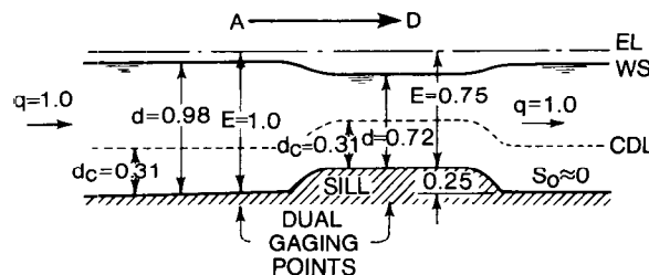
FIGURE 4.—Type III control: subcritical-flow contraction obtained by small increase in bed elevation, horizontal bed (for an explanation of symbols and units, see fig. 2).
